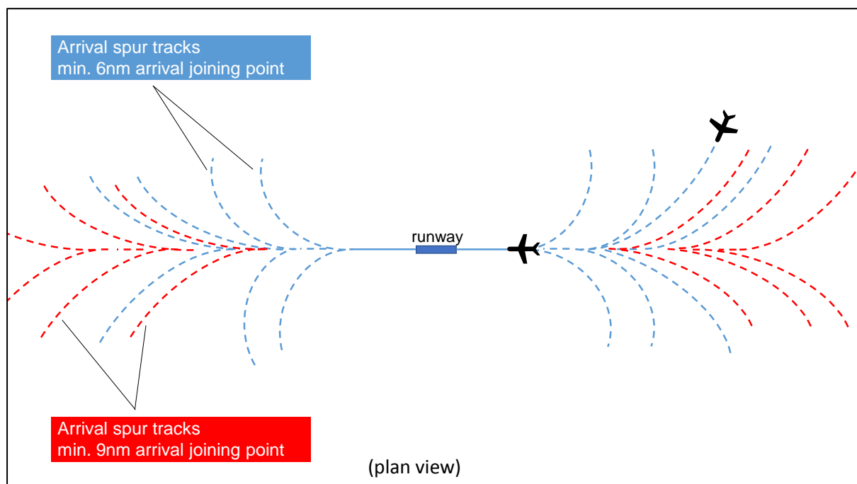
Figure 4: Illustrative example of an air traffic control operational procedure change causing a shift in ILS joining point that could lead to a Type 3 relevant PPR
