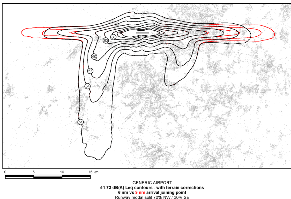
Figure 5: Illustrative example of the change in noise contours caused by a Type 3 relevant PPR
