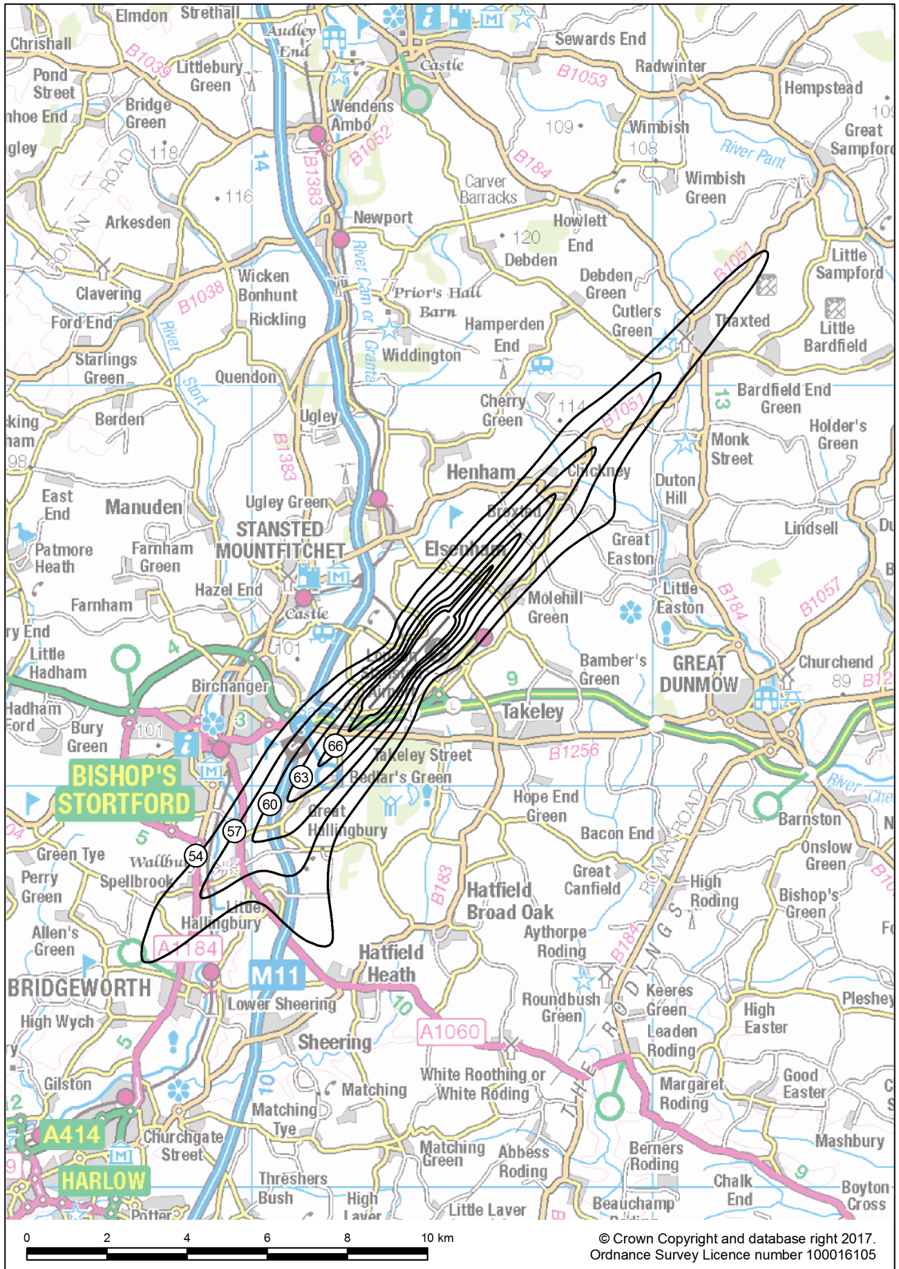
Figure 8 Stansted 2016 annual day L_{Aeq,16hr} 54-69 dBA contours
