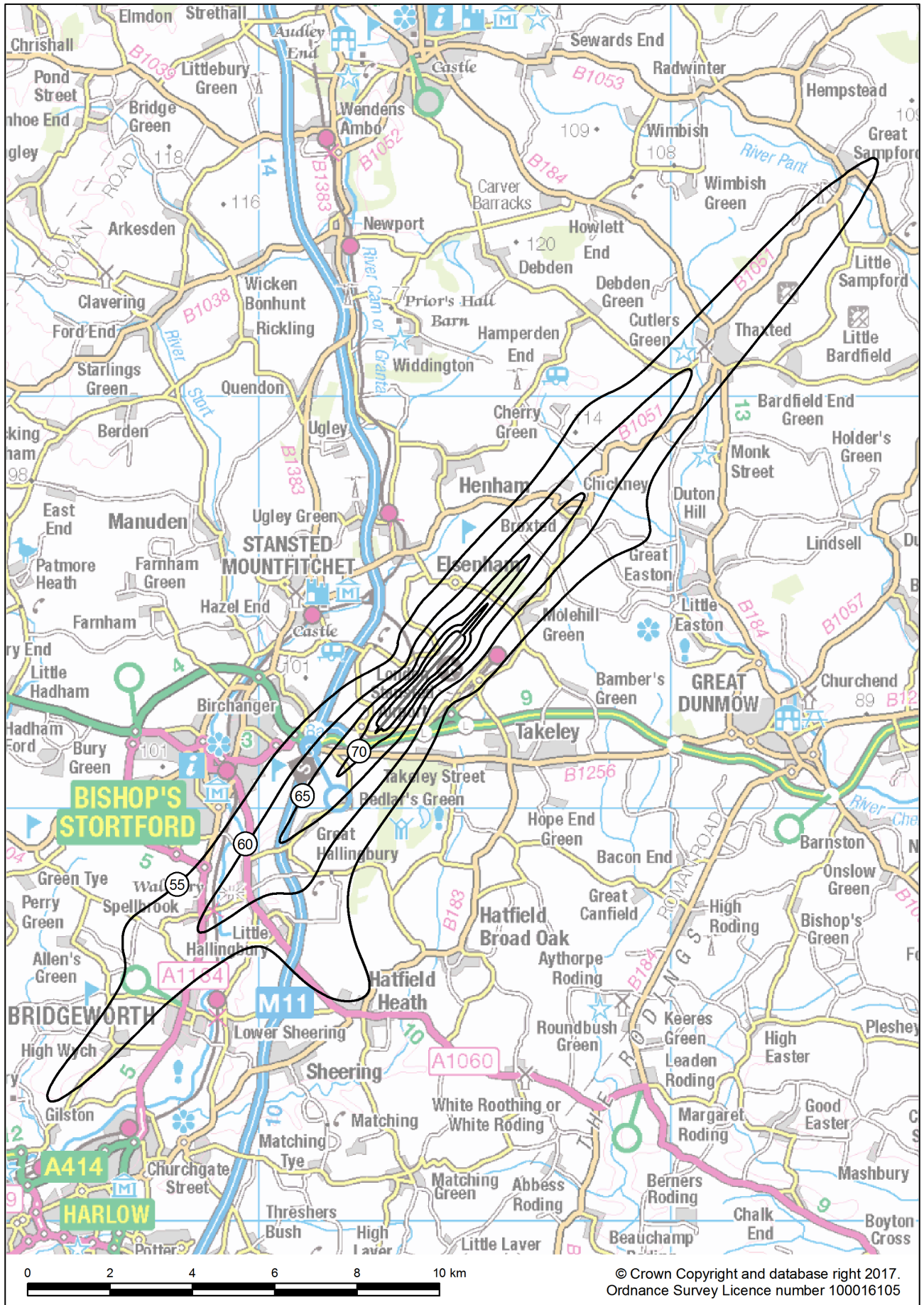
Figure 7 Stansted 2016 L_{den} 55-75 dBA contours
