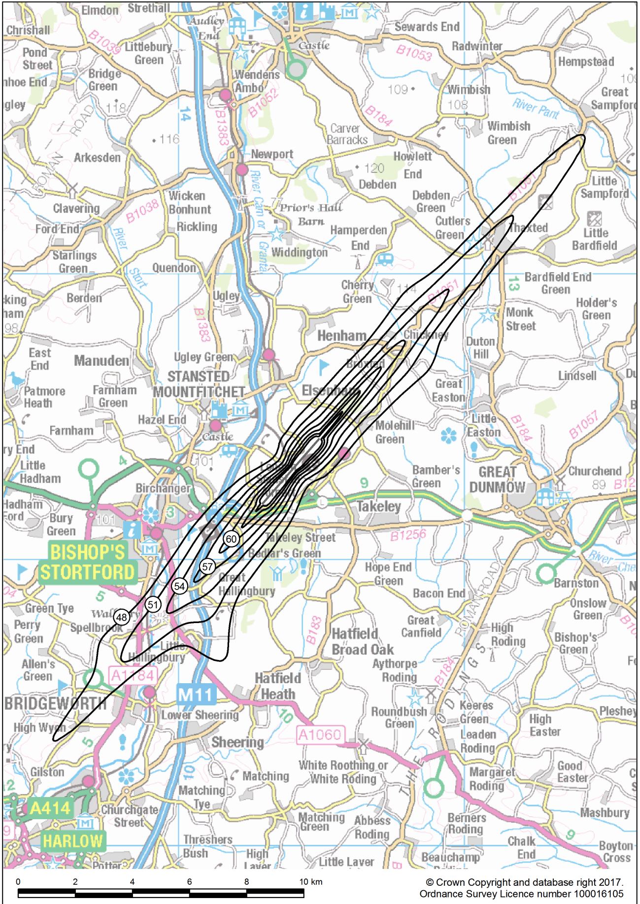
Figure 6 Stansted 2016 L night 48-66 dBA contours
