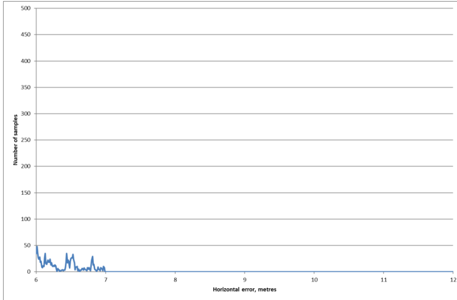
Figure 3-3: Horizontal Error Distribution above 6m for Monitoring Period
