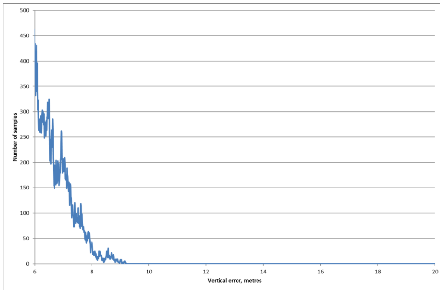
Figure 3-4: Vertical Error Distribution above 6m for Monitoring Period
