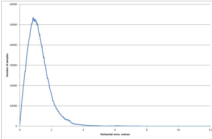
Figure 3-1: Horizontal Error Distribution for Monitoring Period
