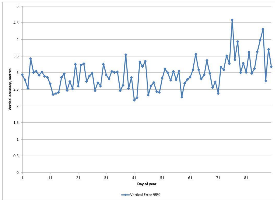
Figure 3-6: Vertical Position Accuracy (95%) for Monitoring Period
