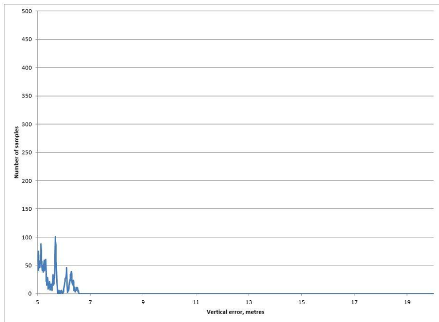
Figure 3-4: Vertical Error Distribution above 5m for Monitoring Period
