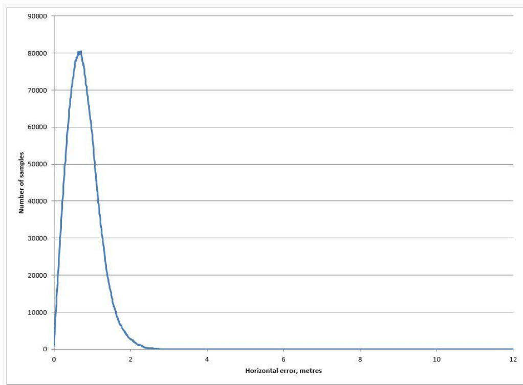
Figure 3-1: Horizontal Error Distribution for Monitoring Period
