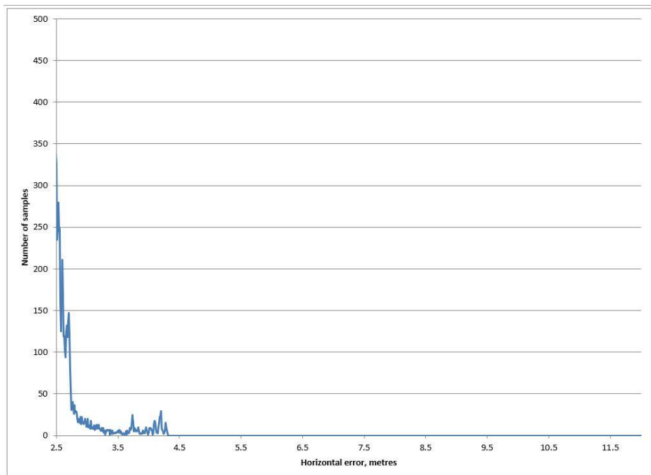
Figure 3-3: Horizontal Error Distribution above 2.5m for Monitoring Period
