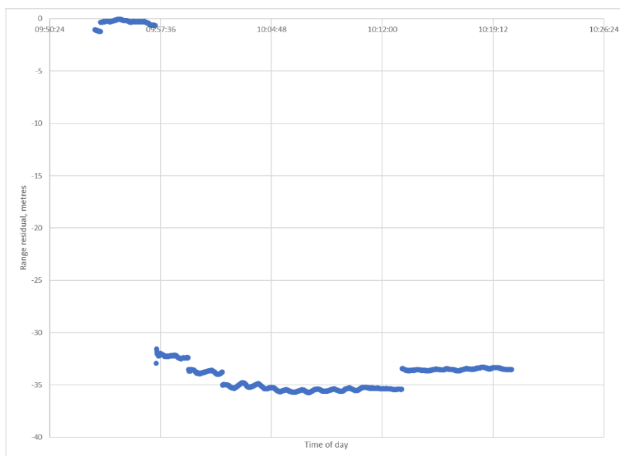
Figure 5-4: Range Residual Error on PRN01 on 10 th July 2023 at NOTT
