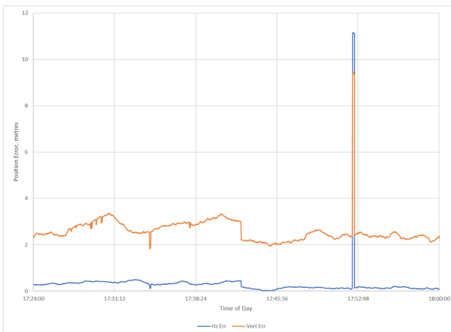
Figure 5-9: Position Error during period of High PRN15 Error on 22 nd August 2023 at NOTT
