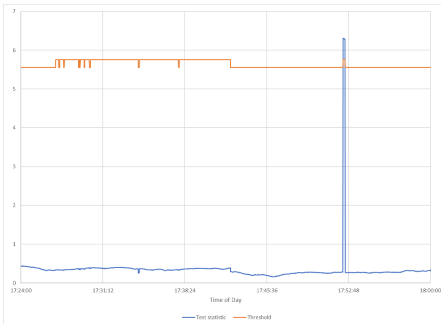
Figure 5-10: RAIM Test Statistic during period of High PRN15 Error on 22 nd August 2023 at NOTT
