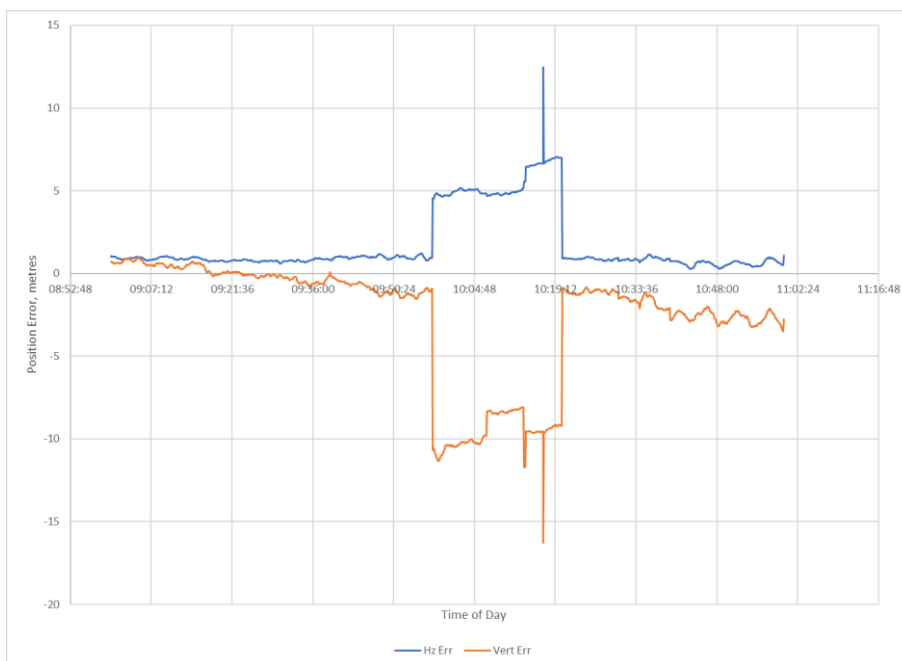
Figure 5-8: Position Error during period of High PRN01 Error on 10 th July 2023 at HARW
