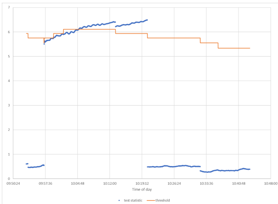
Figure 5-6: RAIM Test Statistic during period of High PRN01 Error on 10 th July 2023 at NOTT
