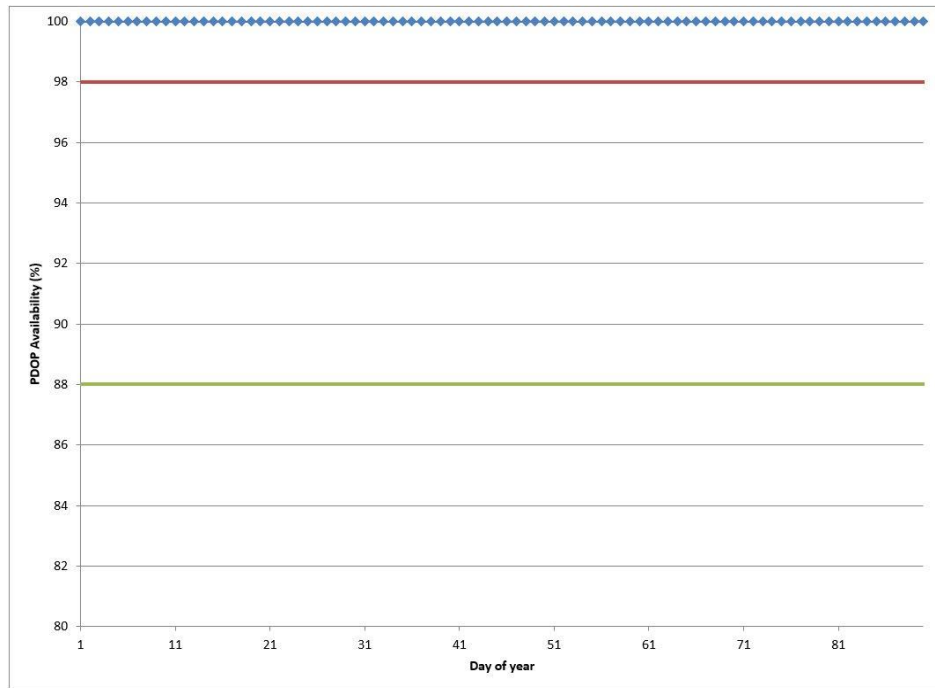
Figure 3-3: Daily PDOP Availability in the Reporting Period
