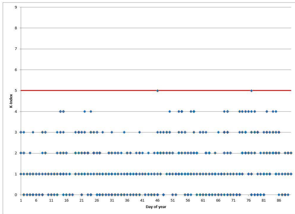
Figure 6-2: K-Index Values at Eskdalemuir during Reporting Period
