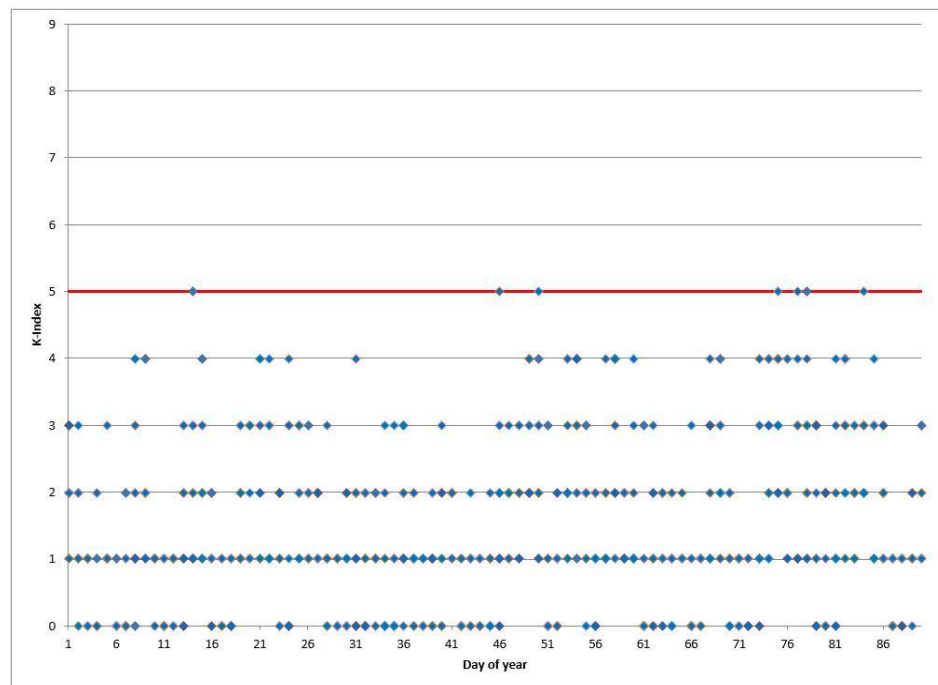
Figure 6-3: K-Index Values at Hartland during Reporting Period
