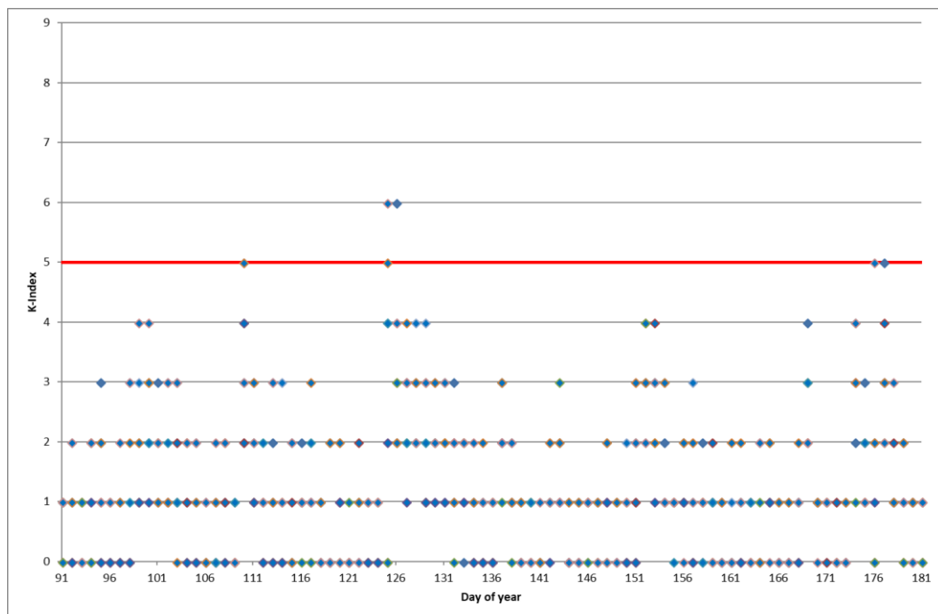
Figure 6-1: K-Index Values at Lerwick during Reporting Period
