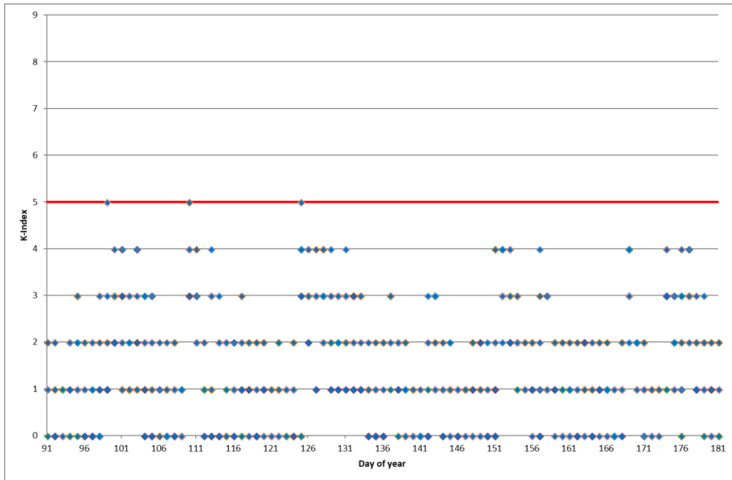
Figure 6-2: K-Index Values at Eskdalemuir during Reporting Period
