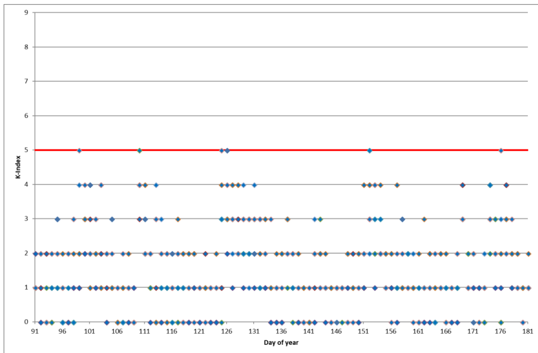
Figure 6-3: K-Index Values at Hartland during Reporting Period
